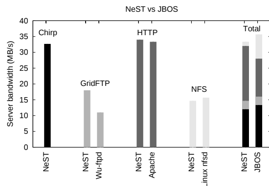
Figure 3. Multiple Protocols. The experiment measures bandwidth when four clients request 10 MB files for each protocol. In the first four sets of bars, only a single protocol is used within each workload (and thus only a single server for JBOS). In the last set of bars, the workload contains all protocols. Within each pair, the first bar shows the performance with NeST and the second bar with JBOS.
