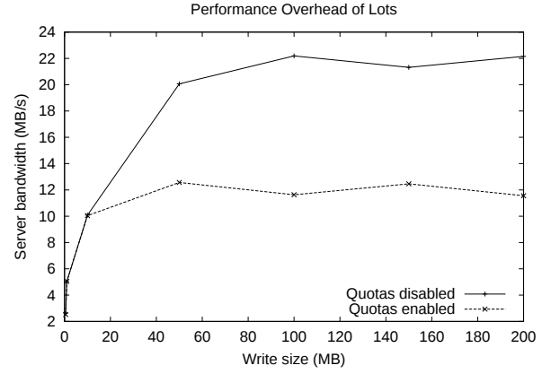
Figure 6. Overhead of lots This graph shows the overhead imposed by implementing lots using the kernel quota system. Notice that for small files, the cost is negligible but increases quickly with file size.
