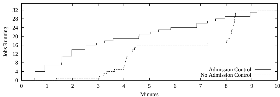
Figure 21: Allocating Network Capacity
