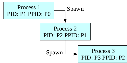
Figure 4. Parent-child relationship
